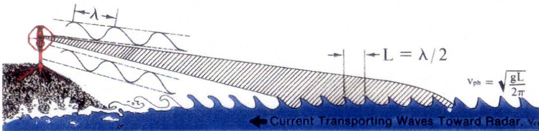
NARROW-BEAM FIRST-ORDER BRAGG SCATTER FROM THE SEA
